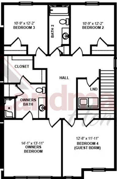
SECOND FLOOR - RIGHT
