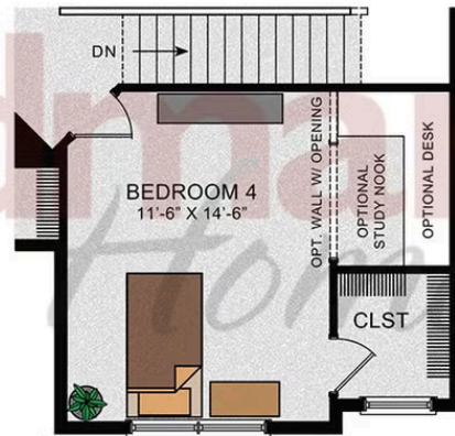
OPTIONAL 4TH BEDROOM ON SECOND FLOOR
